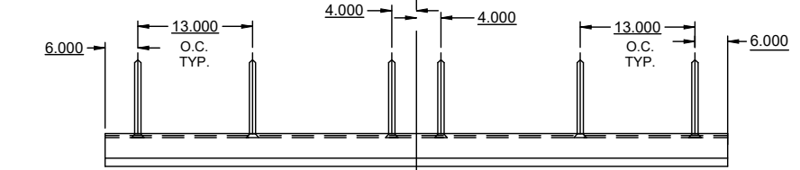
TYPICAL ANCHOR DETAIL AT INTERLOCK OR ASTRAGAL
