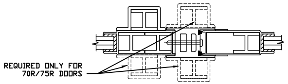
TYPICAL DETAIL AT 2 BY WOOD FRAMING
