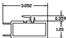
⑰ TOP RAIL/SCREEN WALL THICKNESS 0.062 TYP.
