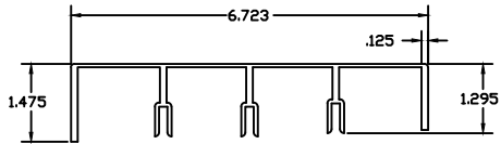
④ THREE TRACK HEAD WALL THICKNESS 0.106
