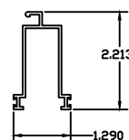
④⁰ HOOK STRIP WALL THICKNESS 0.063 TYP.
