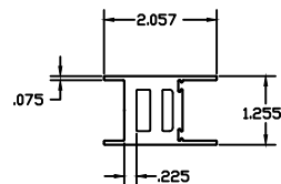
⑮ ASTRAGAL WALL THICKNESS 0.075 TYP.
