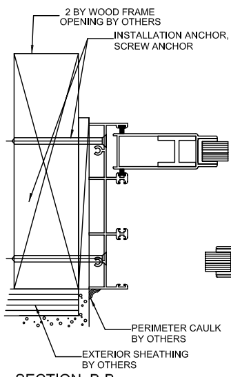
SECTION B-B
