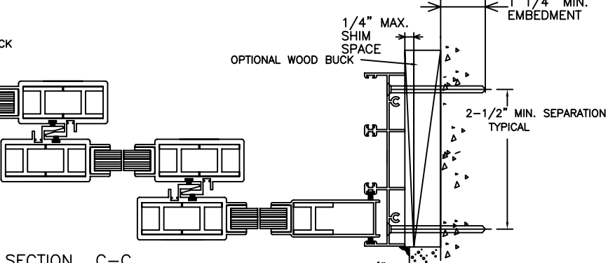
SECTION C-C EXTERIOR INTERLOCK SERIES 50
