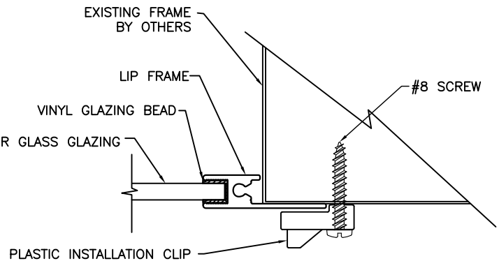
SECTION A GLASS AND ACRYLIC DETAIL
