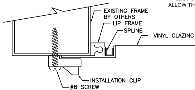
SECTION A VINYL DETAIL
