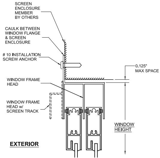
A 1 VERTICAL SECTION 2 TRACK (OUTSIDE MOUNT SHOWN / INSIDE MOUNT SIMILAR)
